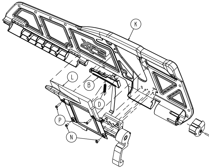
Figure 24 – Release/spring handle assembly components (XPS)
