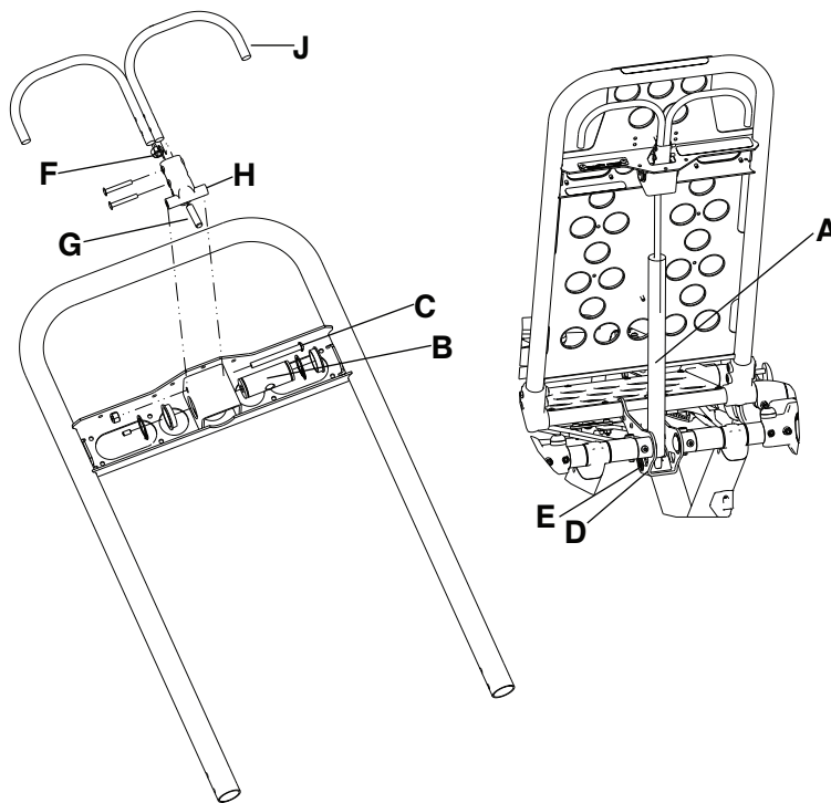
Figure 5 – Backrest
