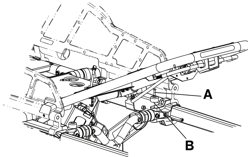
Figure 21 – Siderail assembly replacement (XPS)
