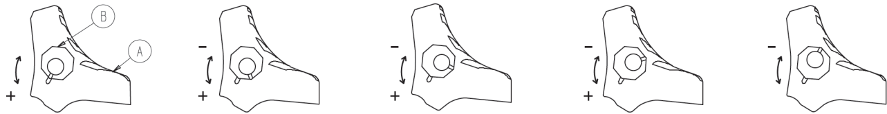
Figure 10 – Wheel locking force adjustment
