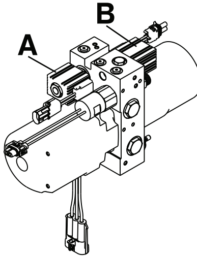
Figure 15 – Hydraulic A valve or B valve replacement
