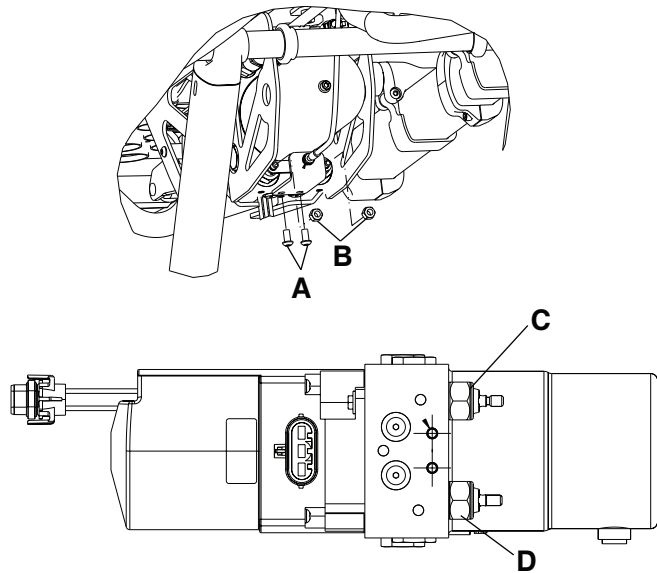
Figure 16 – Hydraulic manual release valve
