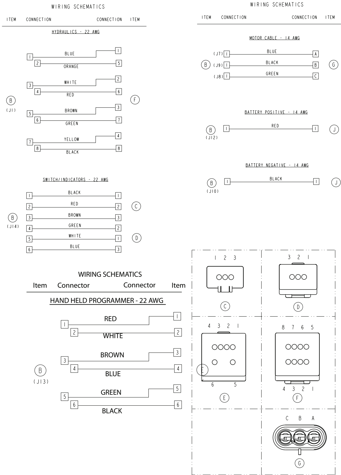
Figure 4 – Wiring Schematics
