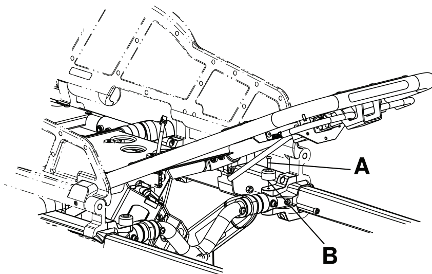
Figure 8 – Siderail assembly replacement (XPS)
