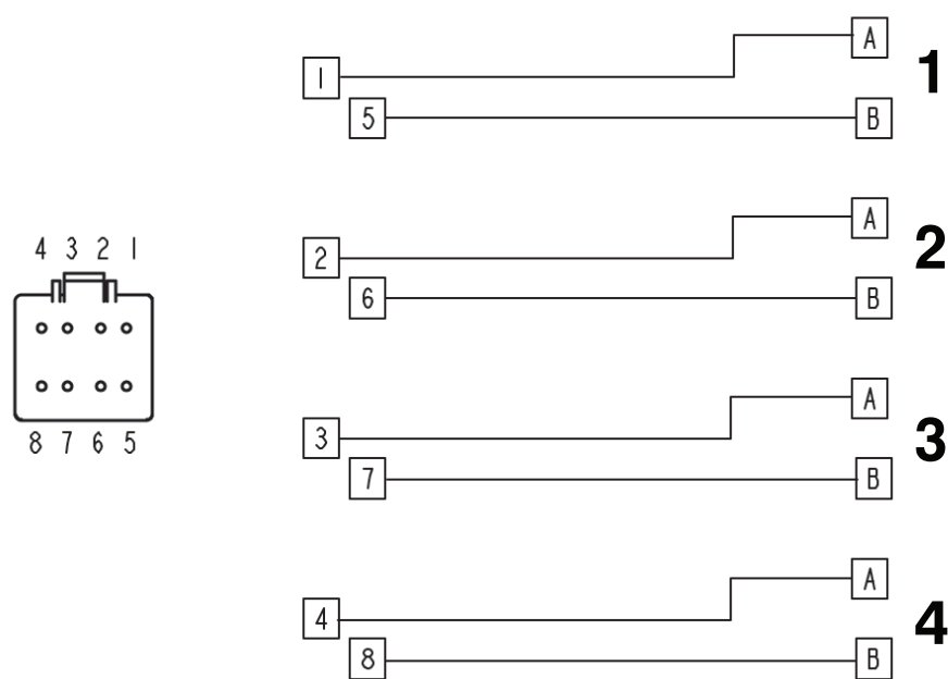
Wiring schematics main cable 8-pin connector
