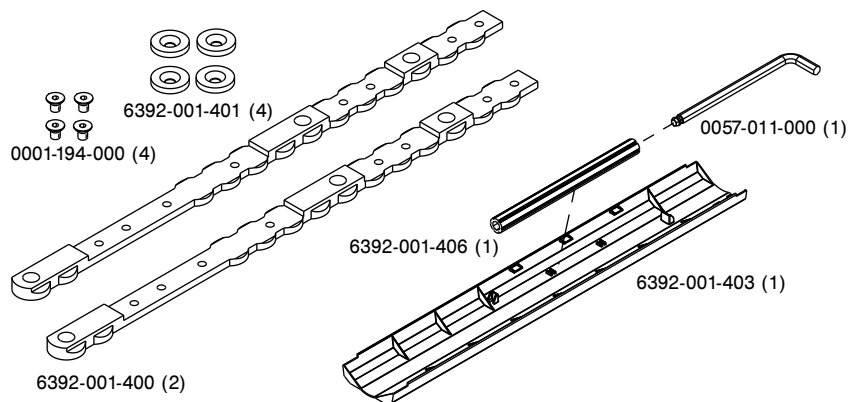
Figur 2 – Performance-LOAD-enhetens kitkomponenter
