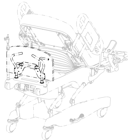
Figure 53 – Replacing the headboard
