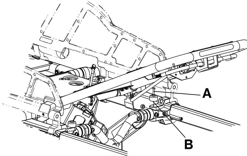
Figure 15 – Siderail assembly replacement (XPS)
