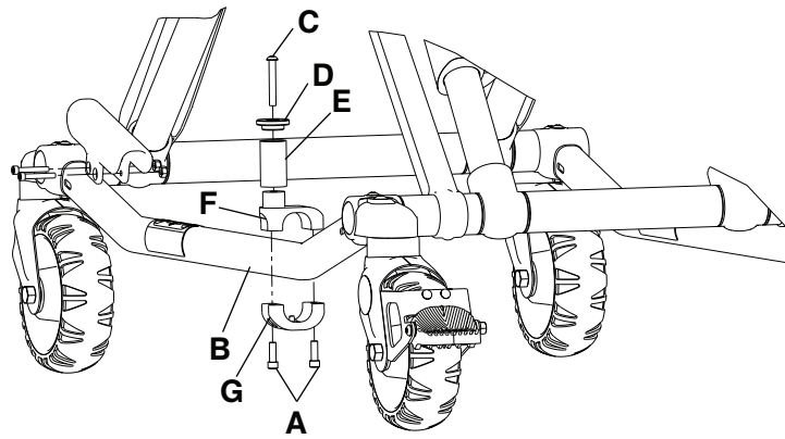
Figure 6 – Cot retaining post replacement
