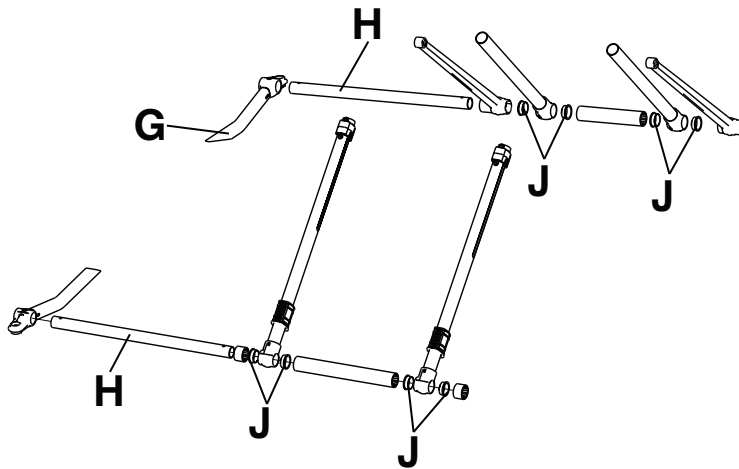
Figure 12 – Disassemble the X-frame
