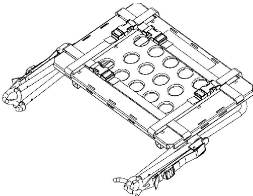
Figure 36 – Stored position
